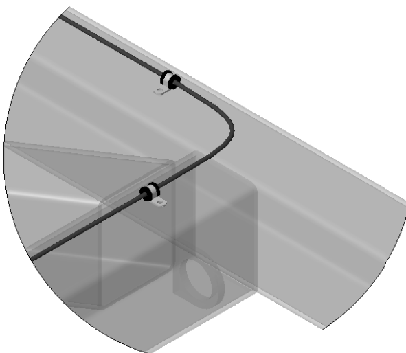
DETAIL E
