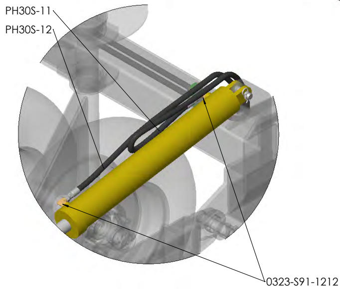
DETAIL G
