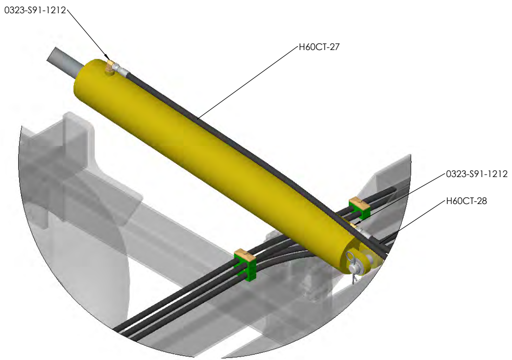
DETAIL D
