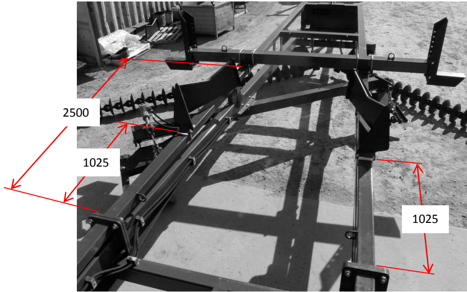
Front Chain Carrier & M Locations
